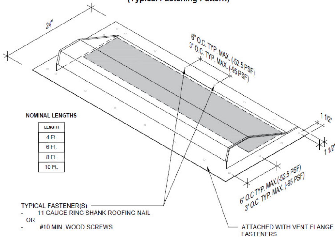
TYPICAL RIDGE VENT ASSEMBLY ISOMETRIC VIEW (Not to Scale)
