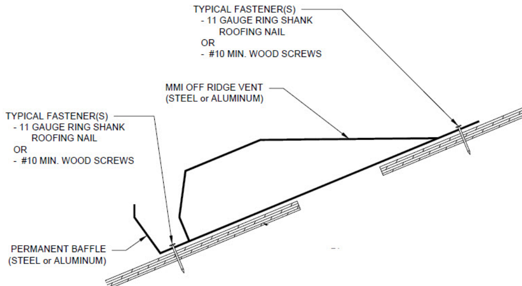
VENT SIDE VIEW (Not to Scale)
