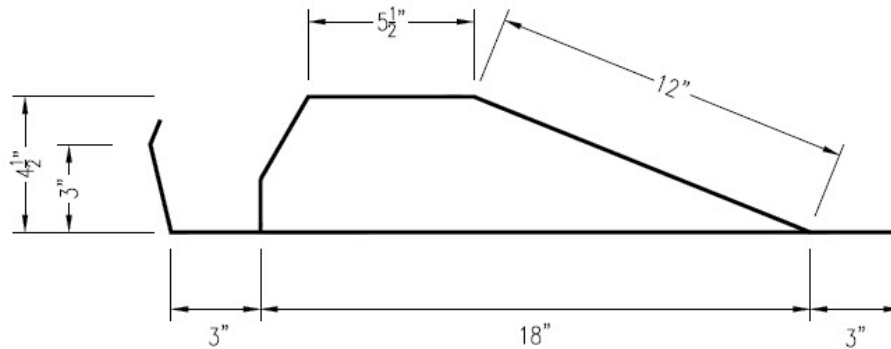
VENT SIDE VIEW (Not to Scale)
