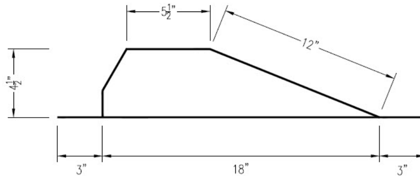
VENT SIDE VIEW (Not to Scale)
